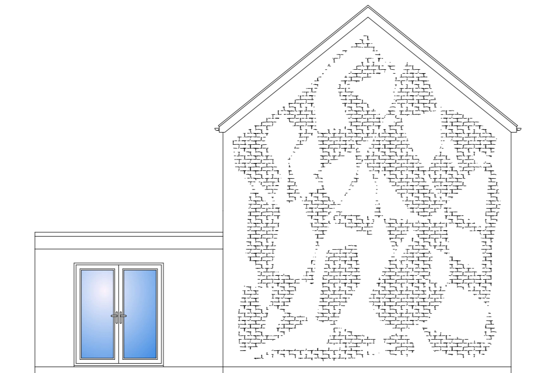
Existing South West Elevation
