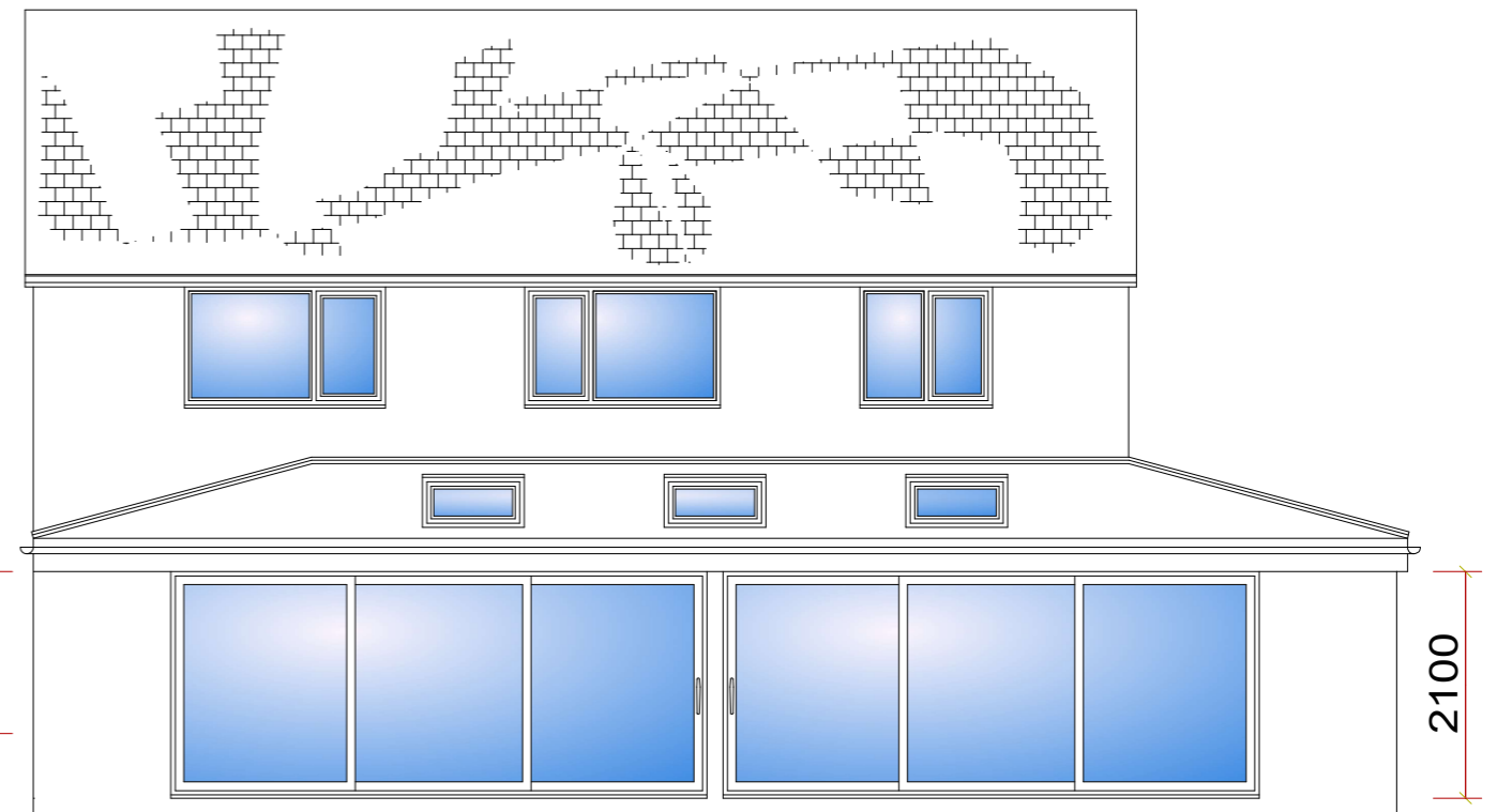
Proposed South East Elevation
