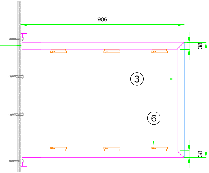
○ Framework: Front Elevation scale 1:12
