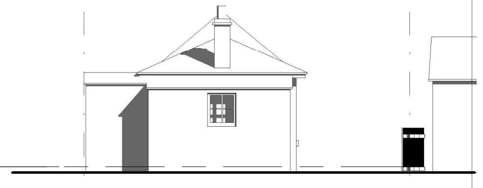
EAST ELEVATION
