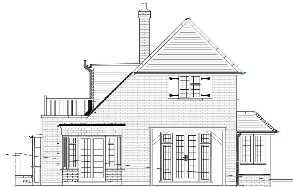
03 EXISTING SIDE ELEVATION
