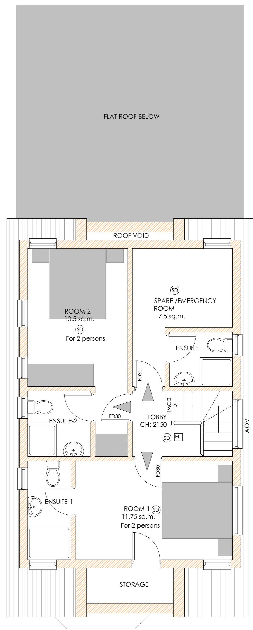
PROPOSED LOFT FLOOR PLAN
