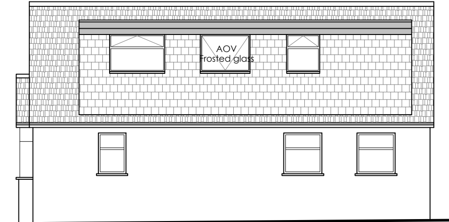
EXISTING OPPOSITE SIDE ELEVATION
