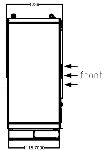
left view
