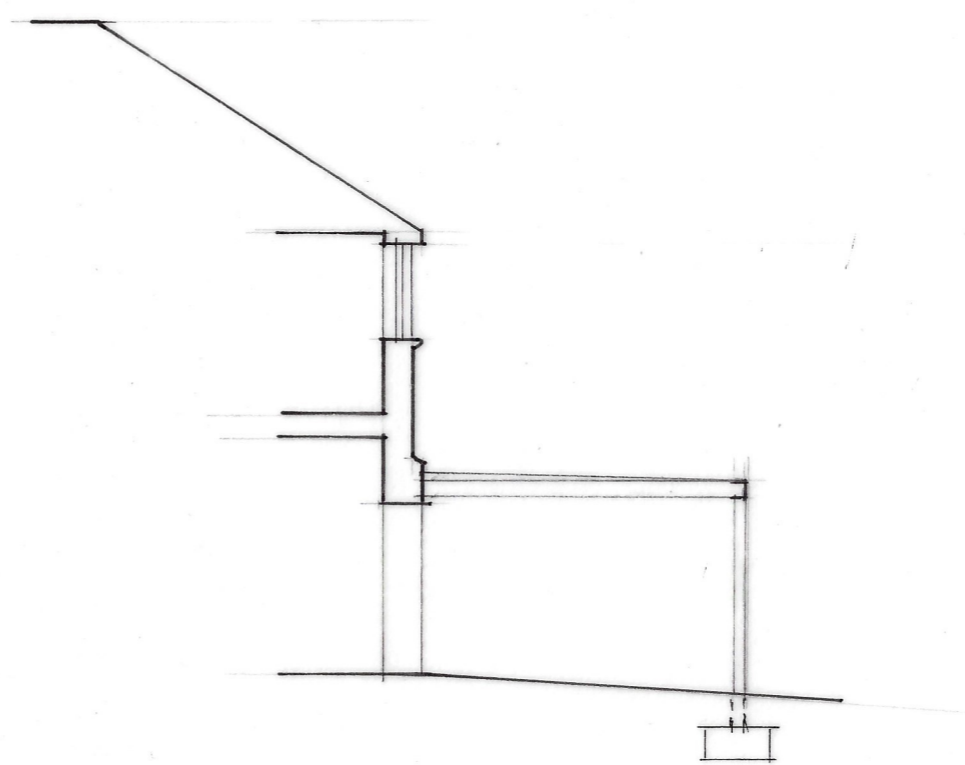
SECTION A
