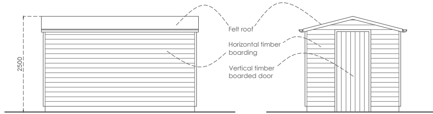
North Elevation
