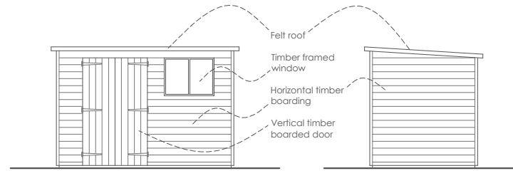
North Elevation
