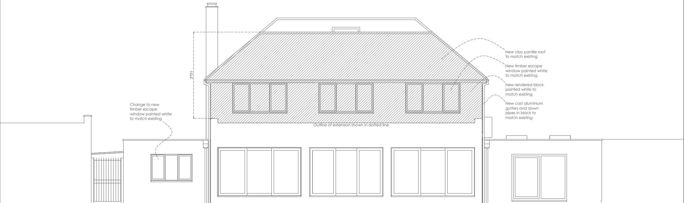
East Elevation
