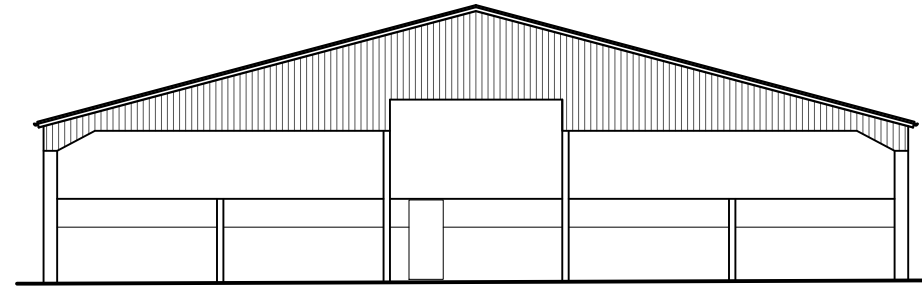
Front Elevation
