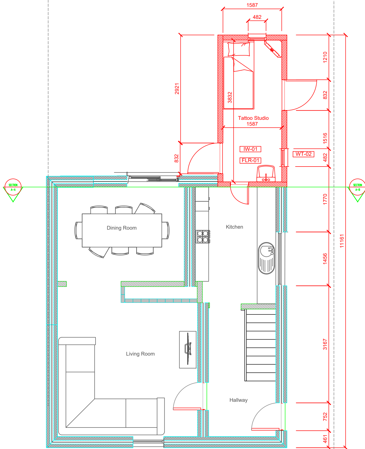
Proposed Ground Plan Scale 1:50@A1-1:100@A3
