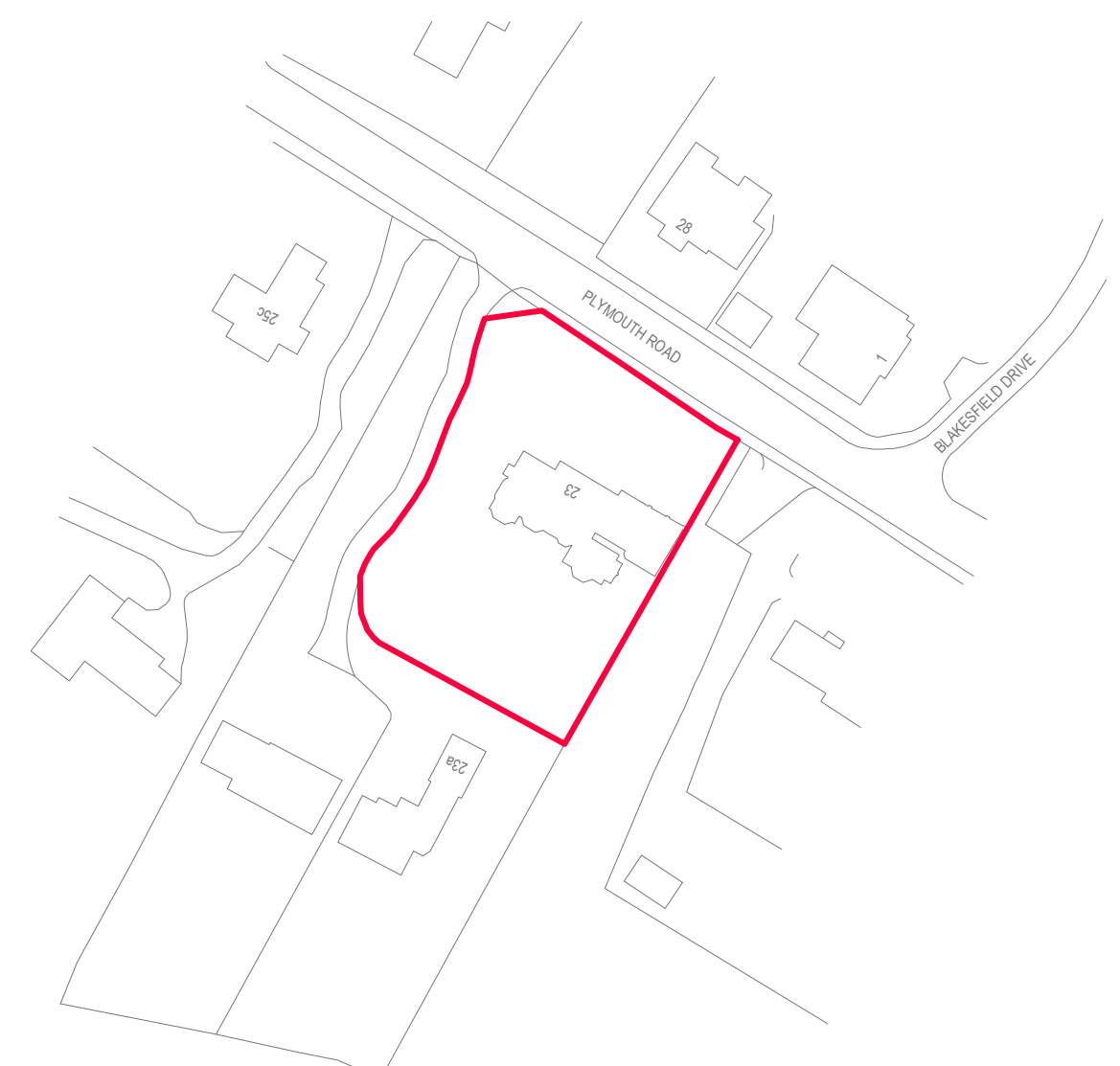
SITE LOCATION PLAN 1:1250 AS EXISTING
