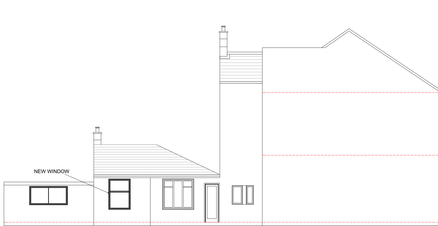
PROPOSED NORTH SECTIONAL ELEVATION
