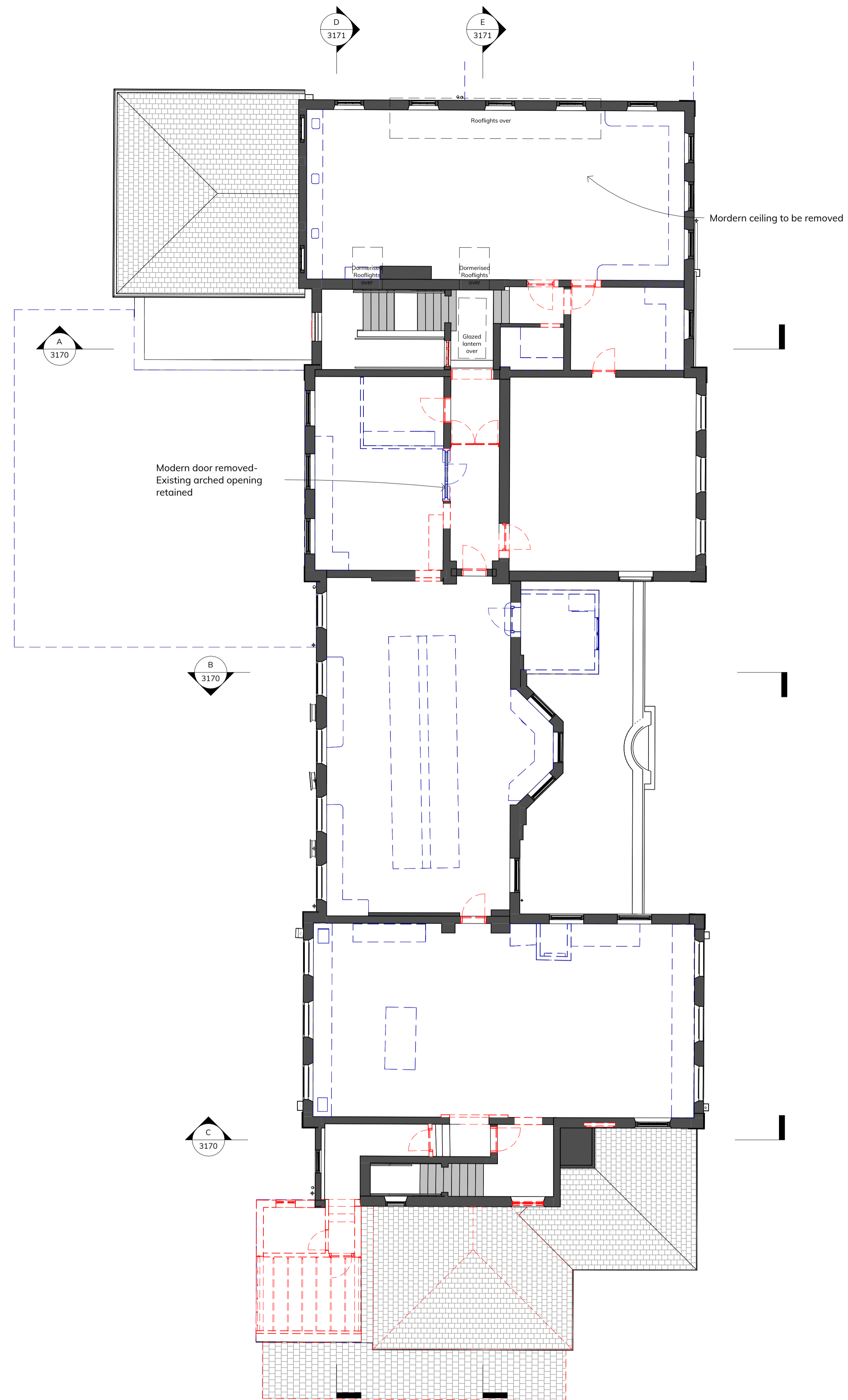
1 GA First Floor Plan - Demolition 1:100
