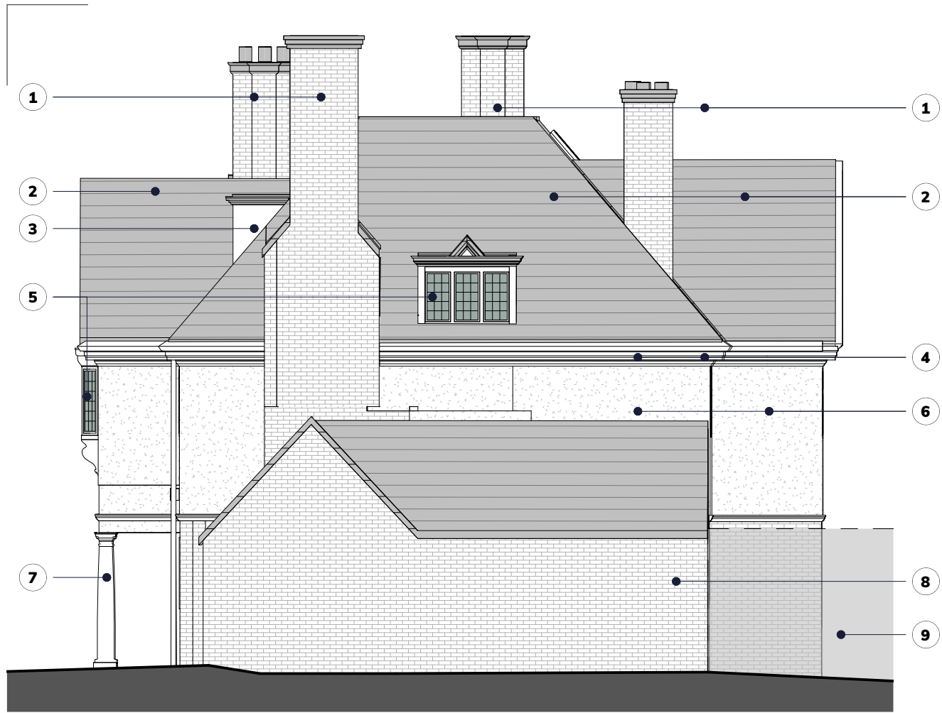
W GA Elevation West - Existing 1 : 100
