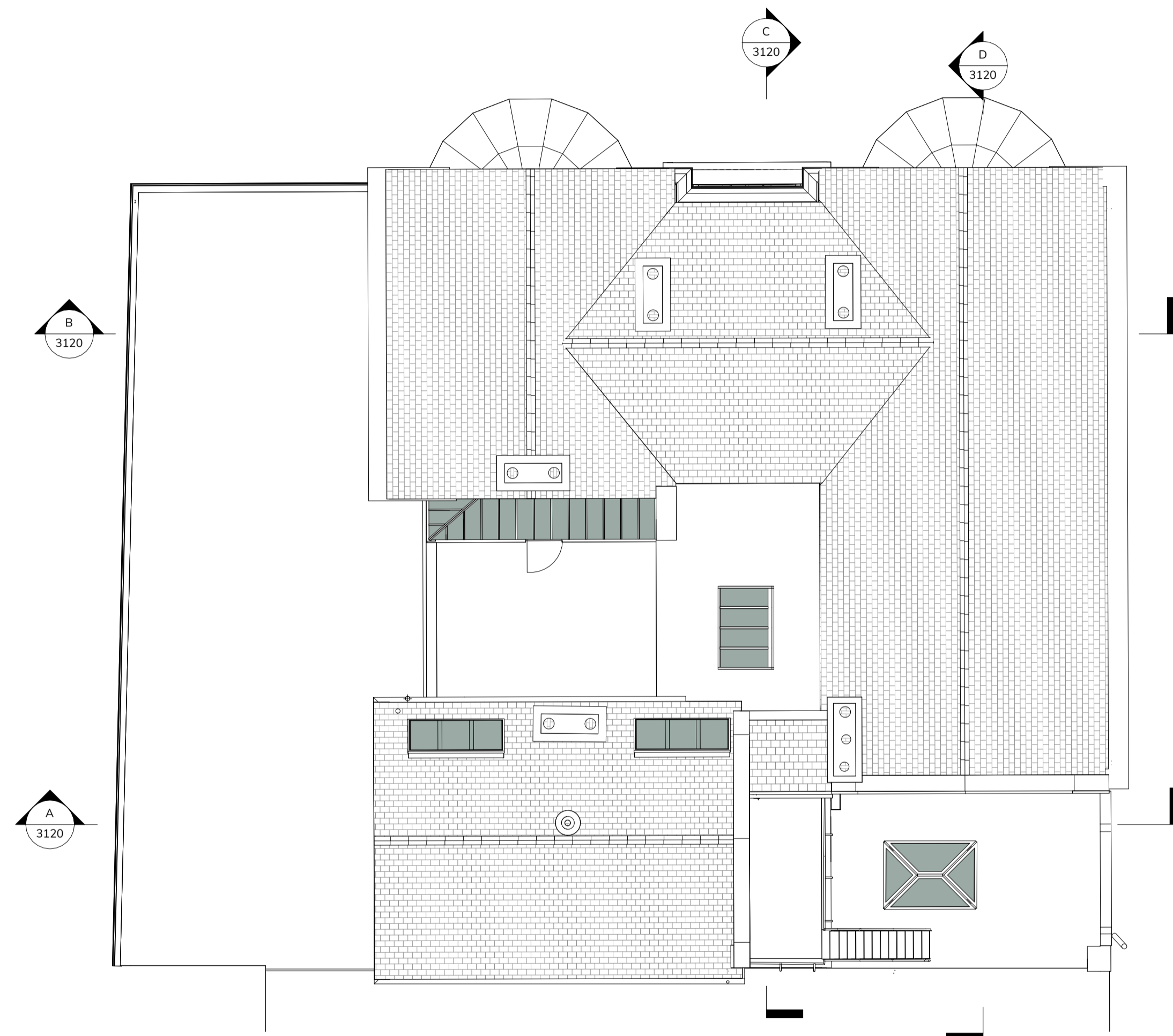
R GA Plan Level R1 Roof Existing 1:100
