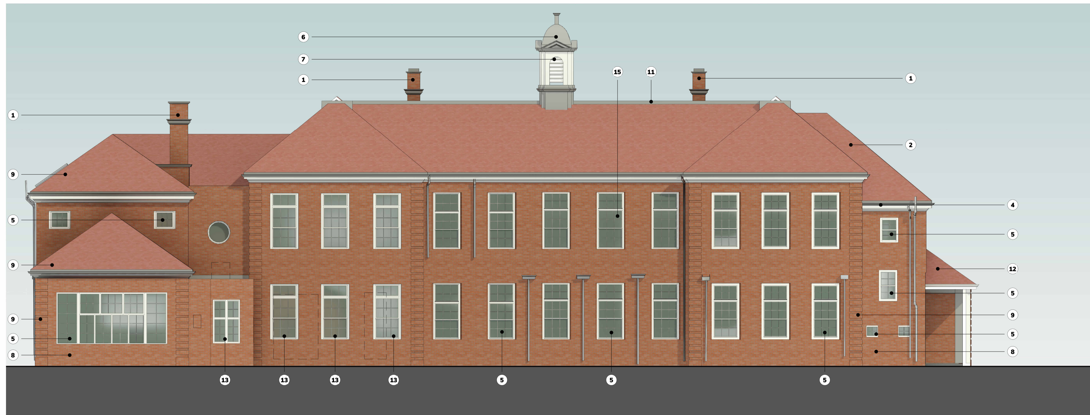
W GA Elevation West Proposed 1:100
