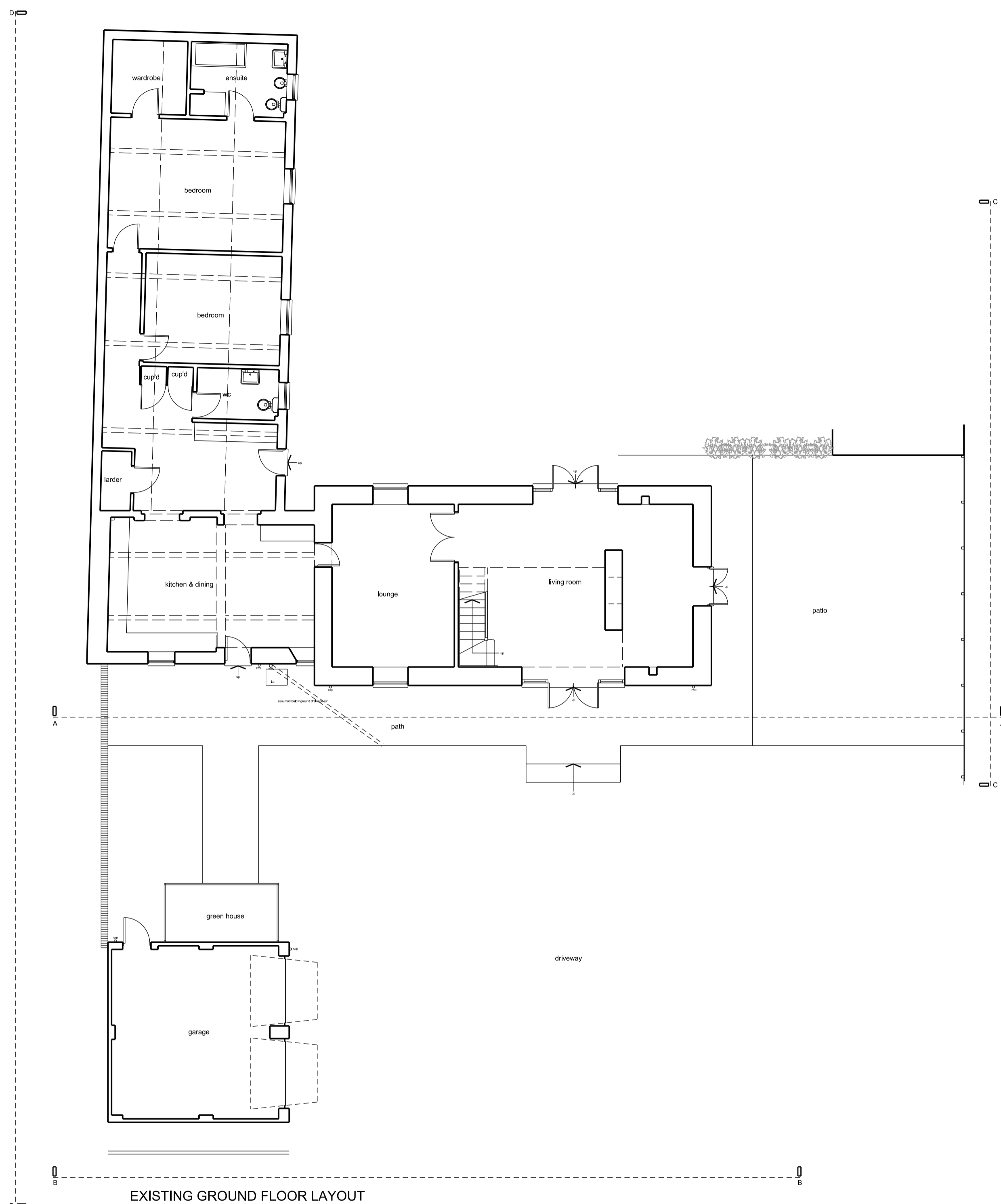
EXISTING GROUND FLOOR LAYOUT
