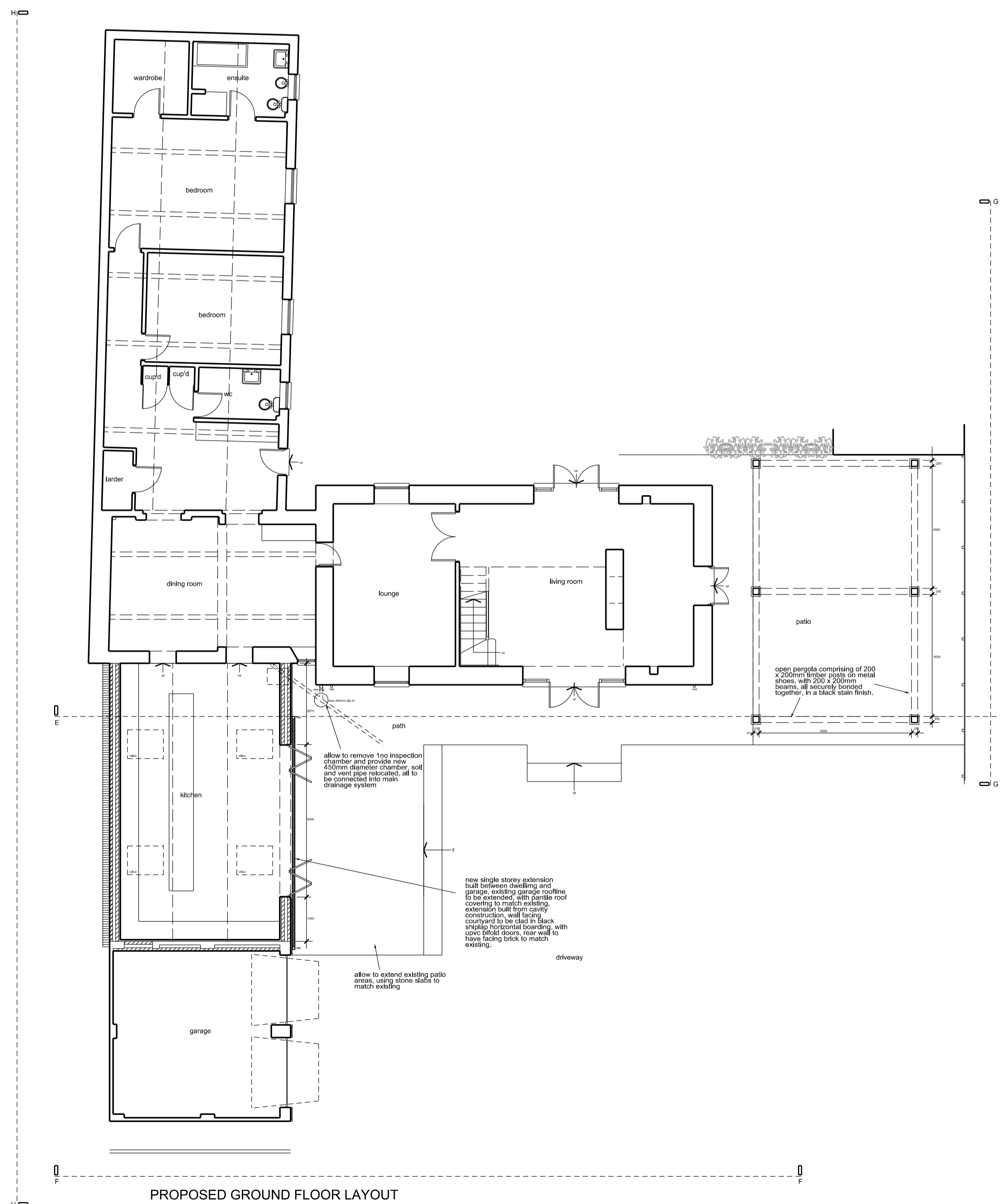
PROPOSED GROUND FLOOR LAYOUT
