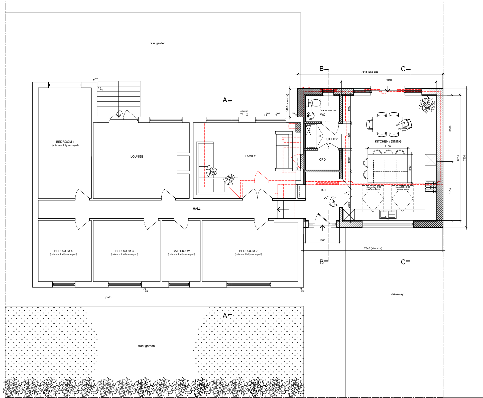
Ground Floor Plan - Proposed - 1:100
