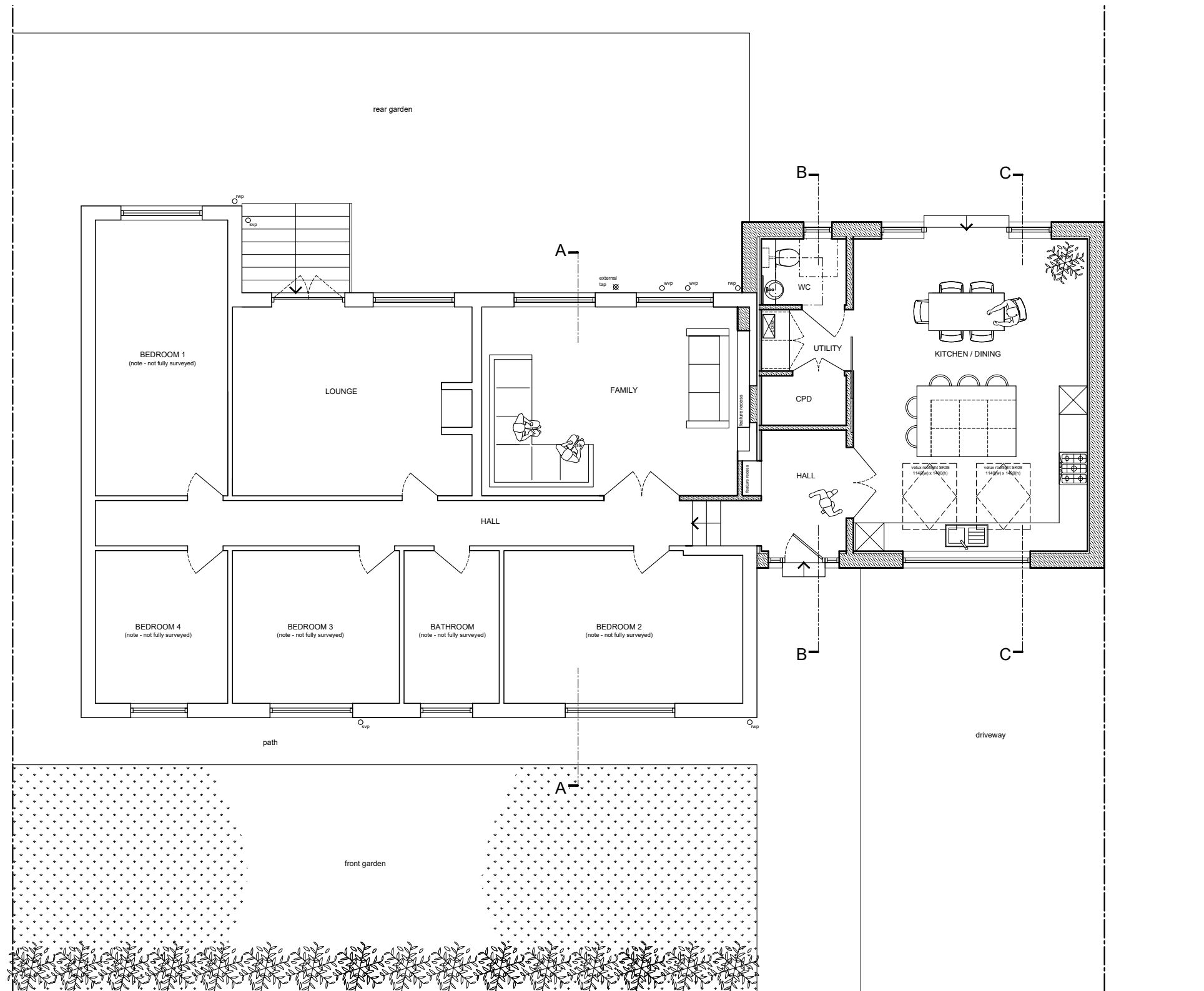
Ground Floor Plan - Proposed - 1:100 Note: Dimension and Demolition layers not shown for clarity
