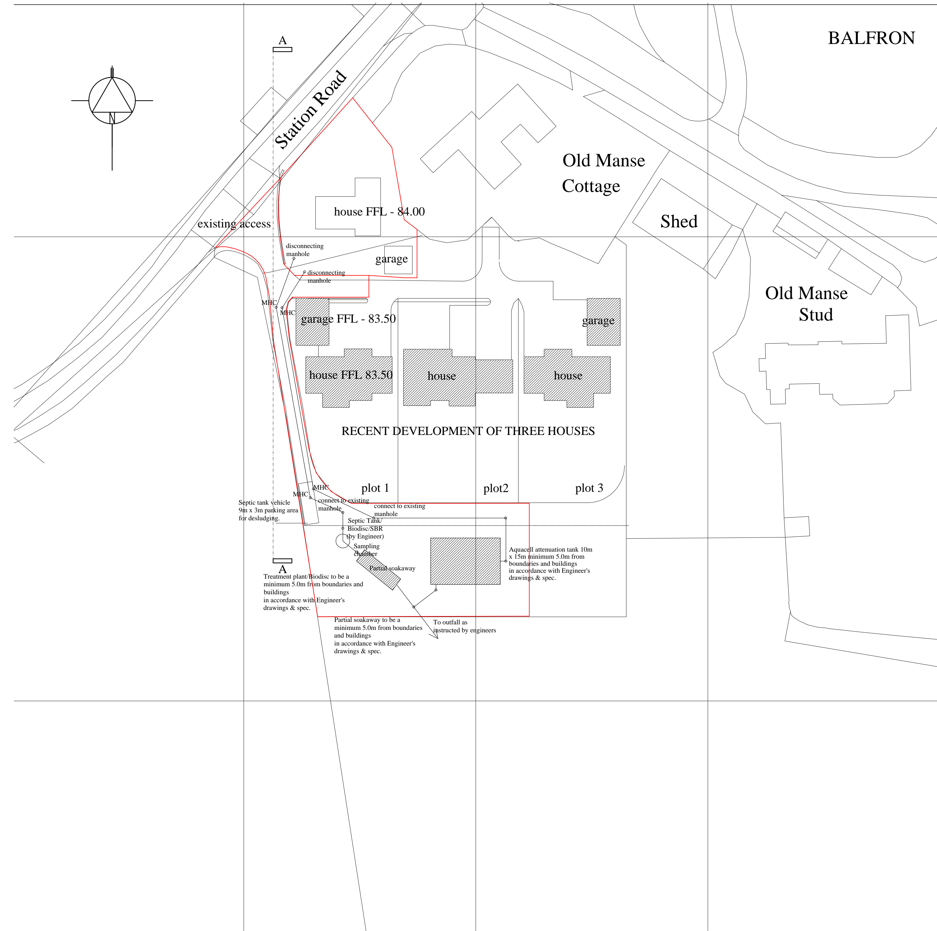
Site Plan 1:500 copyright - ukplanning maps/studioKarchitects
