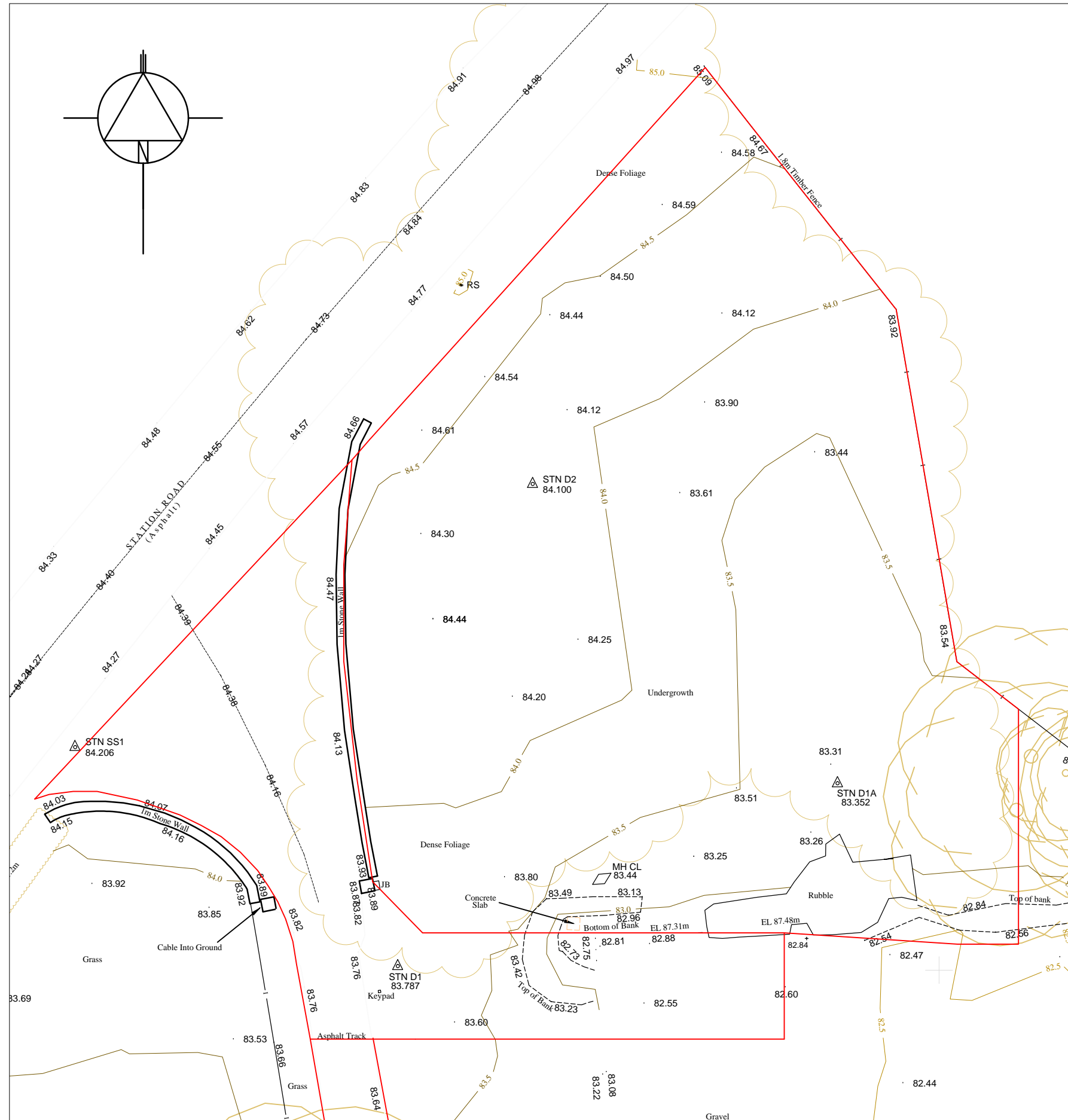
Existing Site Plan & Site Levels 1:200
