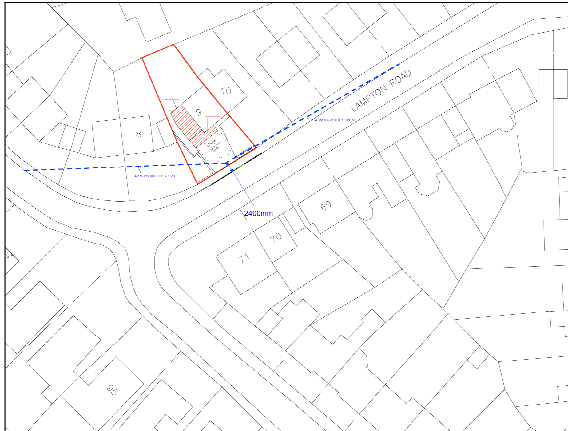
Visibility Splay Plan SCALE 1:200
