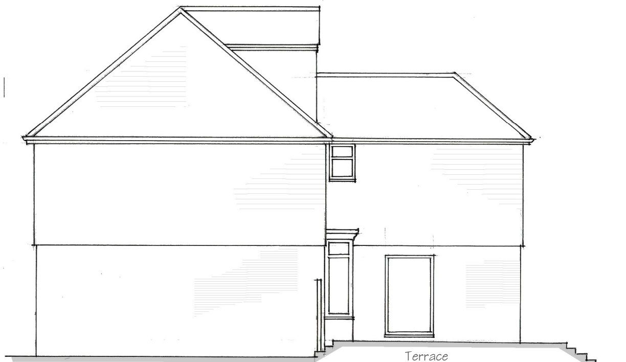
NORTH ELEVATION
