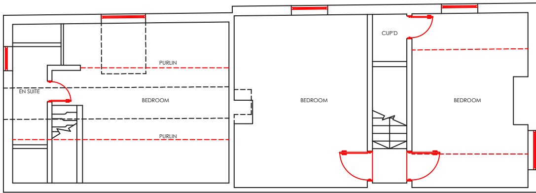
EXISTING FIRST FLOOR PLAN OLDE BARN COTTAGE
