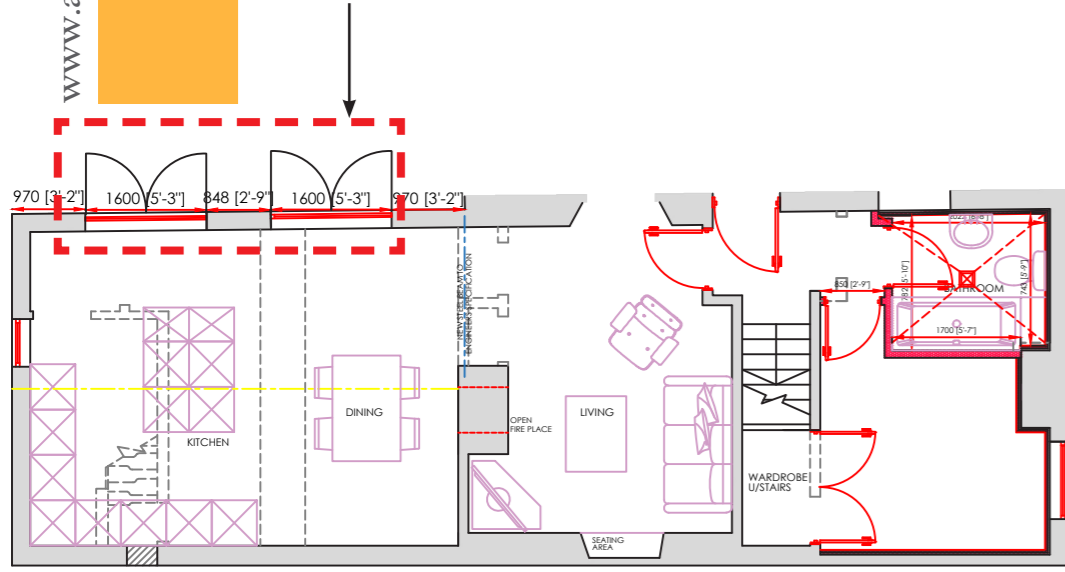
PROPOSED GROUND FLOOR PLAN OLDE BARN COTTAGE
