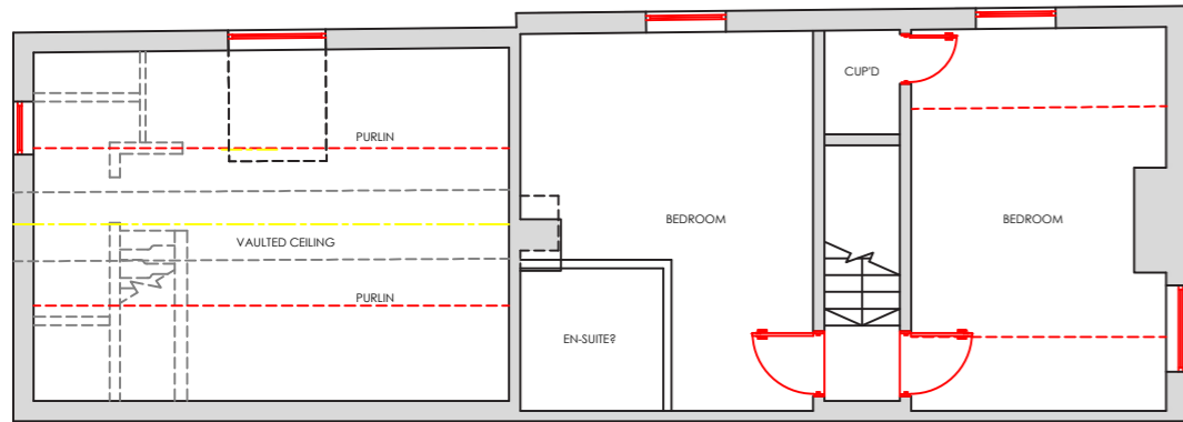
PROPOSED FIRST FLOOR PLAN OLDE BARN COTTAGE
