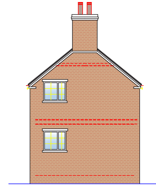
PROPOSED SIDE ELEVATION OLDE BARN COTTAGE
