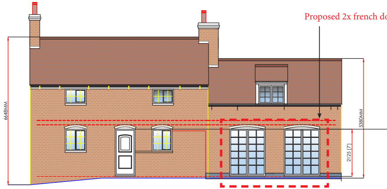
PROPOSED FRONT ELEVATION OLDE BARN COTTAGE
