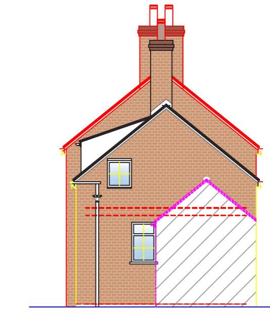
PROPOSED SIDE ELEVATION OLDE BARN COTTAGE
