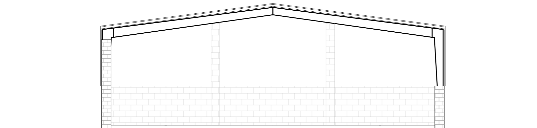
Section B-B
