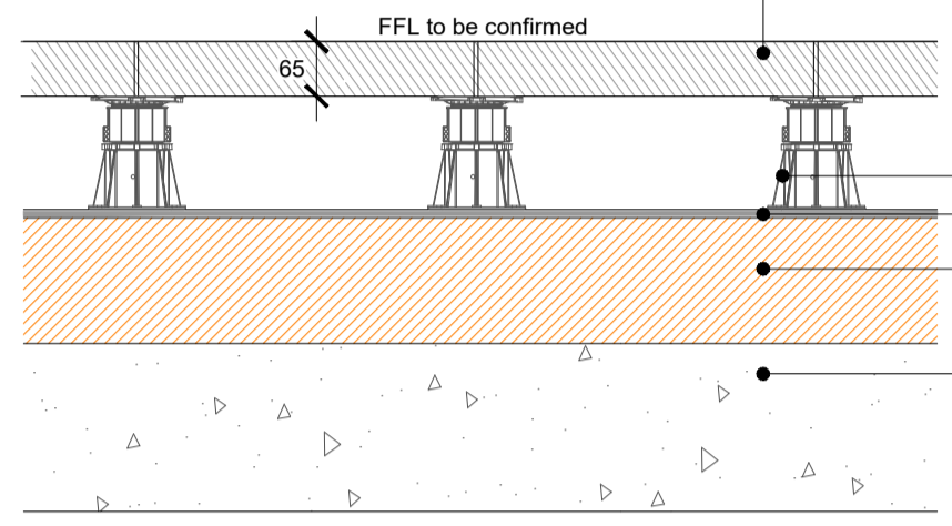
07 Surface type 7 - Permeable PCC Flags to podium 502 Typical detail SCALE 1:10
