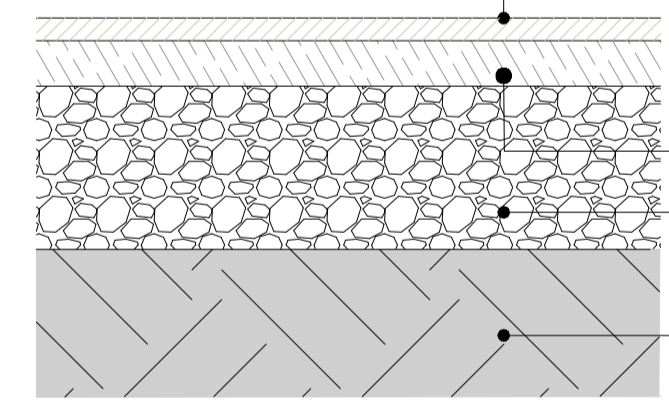
14 Surface type 14 - Permeable wet pour / Coloured macadam surfacing to play areas 502 Typical detail SCALE 1:10
