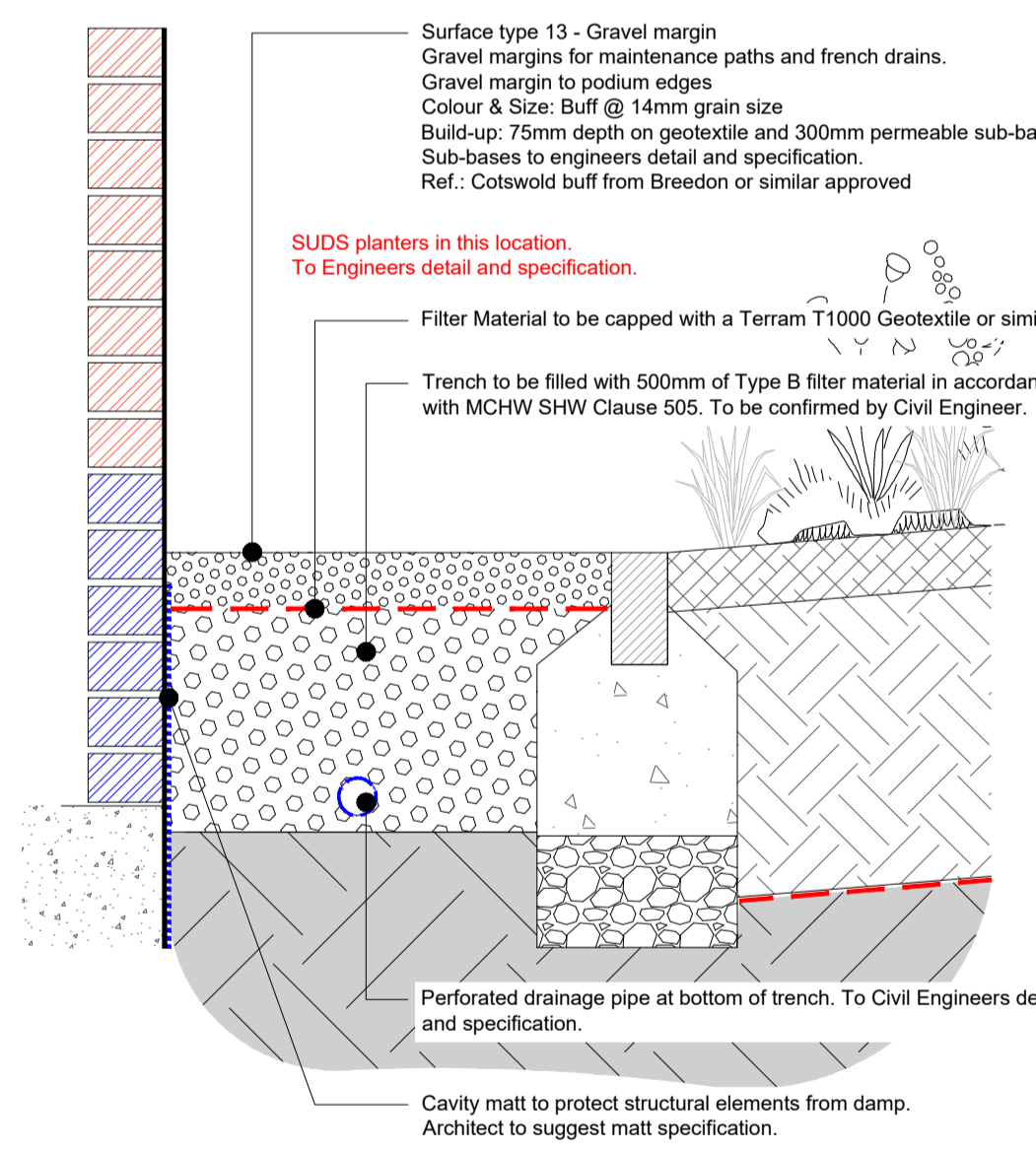
13 Surface type 13 - Gravel margin 502 Typical detail SCALE 1:10
