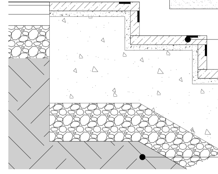
01 Surface type 12 - Steps 503 Typical detail SCALE 1:10
