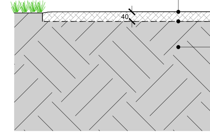
10 Surface type 10 - Rubber mulch matt for running 502 Typical detail SCALE 1:10
