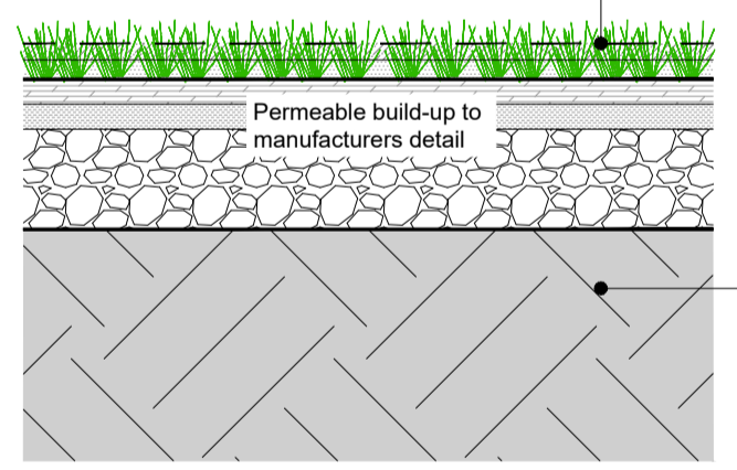
11 Surface type 11 - Artificial turf to infant MUGA 502 Typical detail SCALE 1:10
