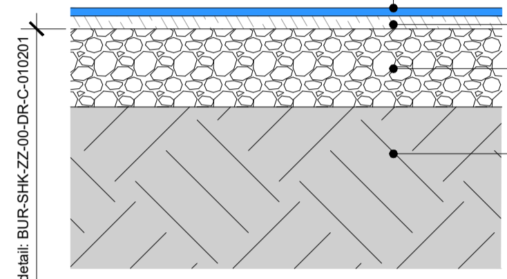
08 Surface type 8 - Wet pour surfacing to play areas 502 Typical detail SCALE 1:10
