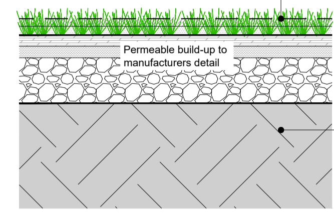
09 Surface type 9 - Artificial turf to Junior MUGA 502 Typical detail SCALE 1:10
