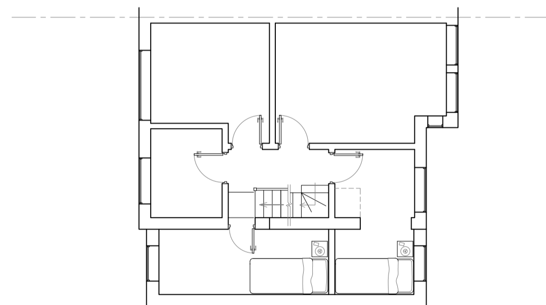
Proposed First Floor GA
