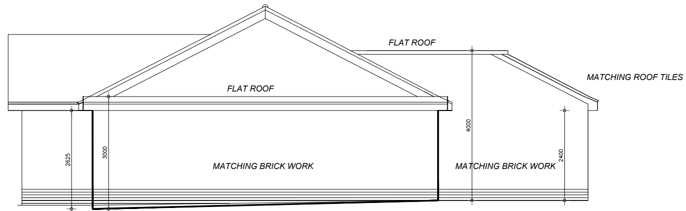
PROPOSED SIDE ELEVATION (north)
