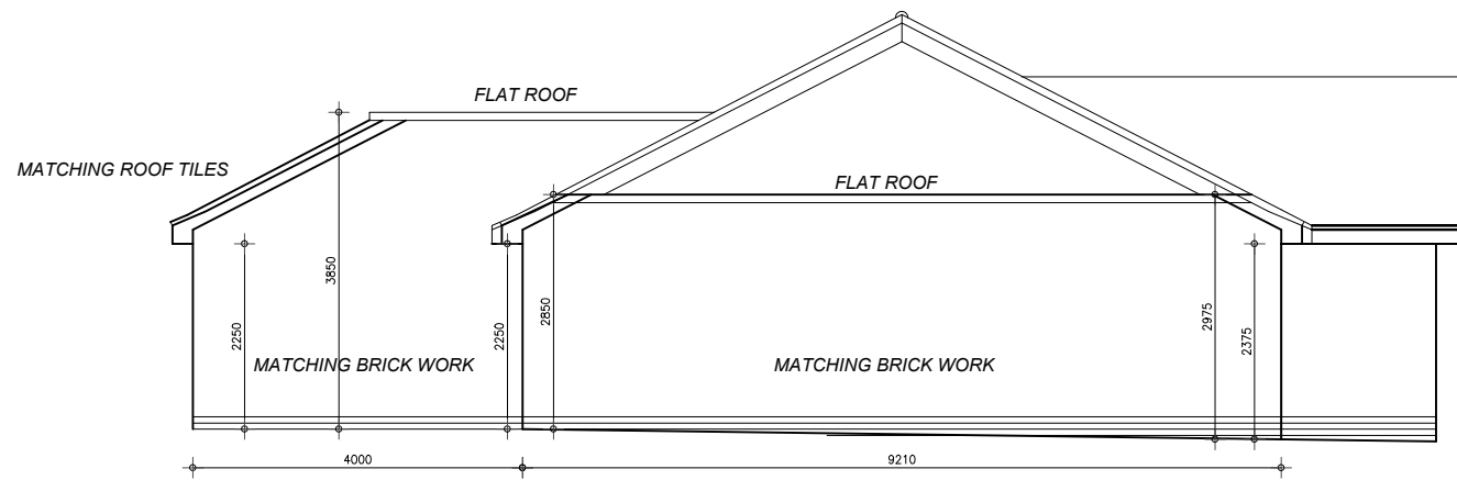
PROPOSED SIDE ELEVATION (south)
