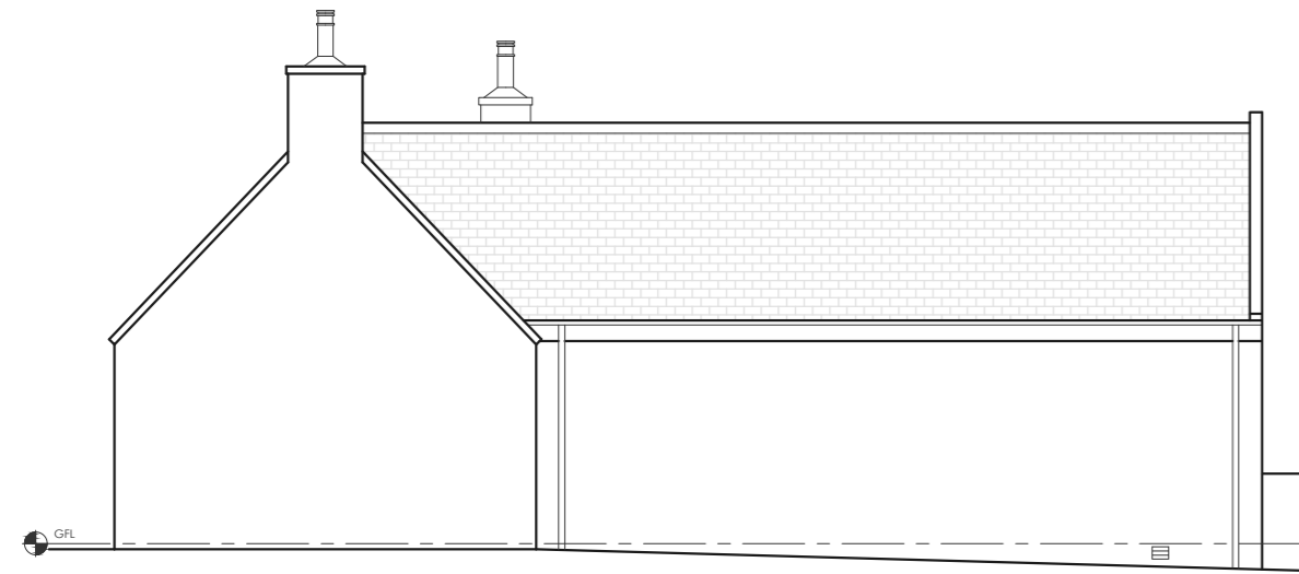
North Elevation 1:100
