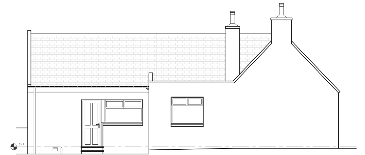
South Elevation 1:100
