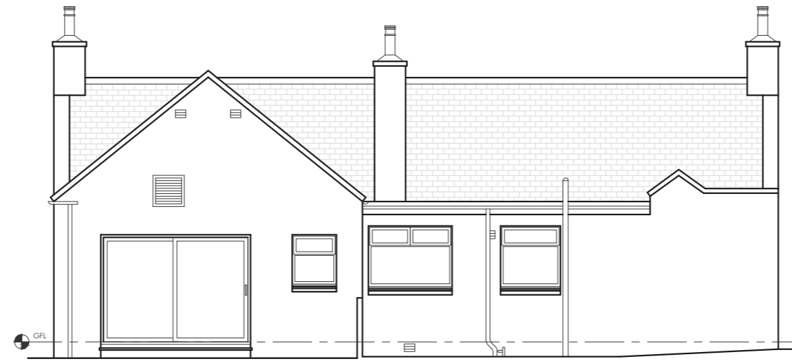
West Elevation 1:100
