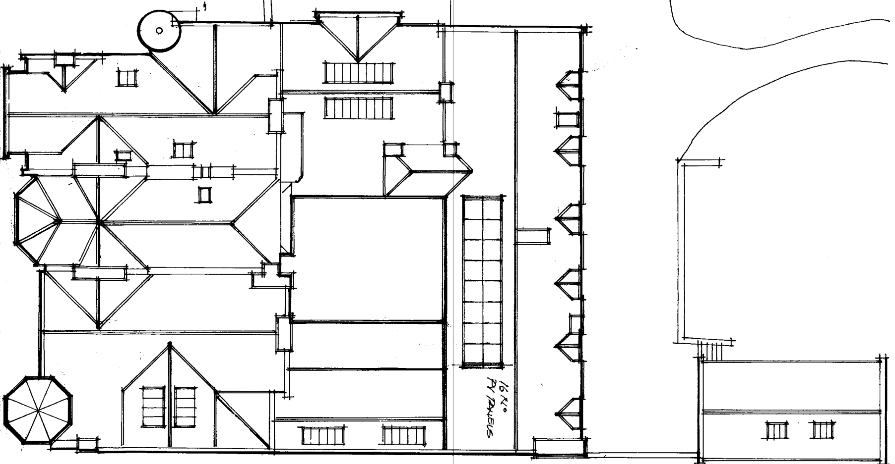
Block/roof plan 1:200
