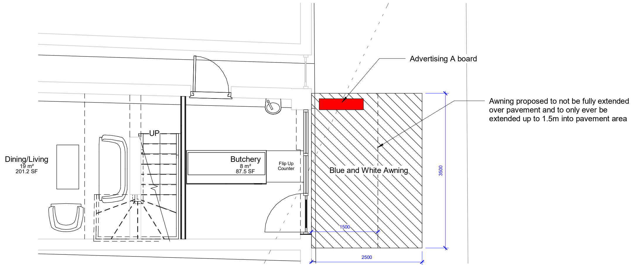
1 Proposed Ground Floor - Awning and Advertising 1 : 50
