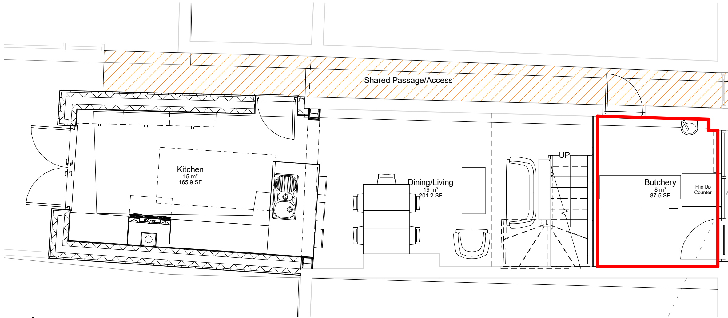
1 Proposed Ground Floor - Change of Use 1 : 50
