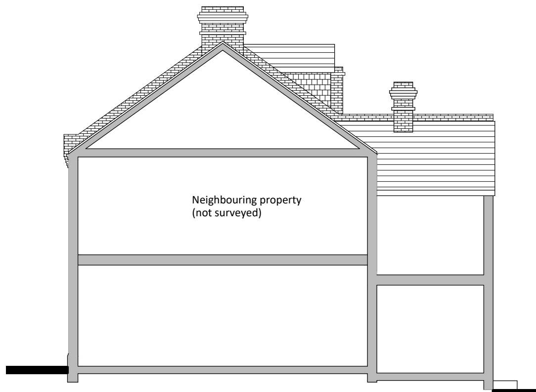
Existing Indicative Side Elevation / Section Scale 1:100
