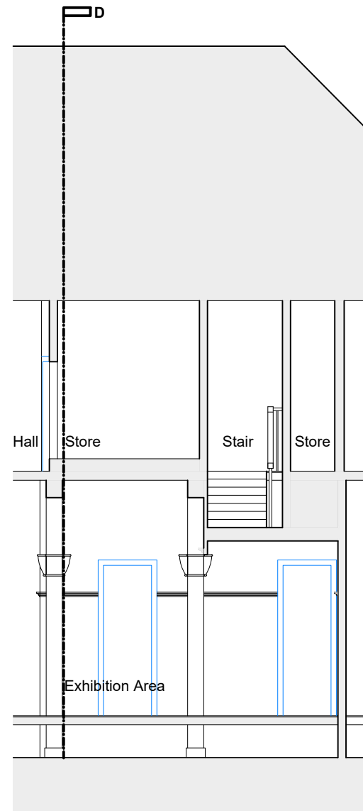
01 Section E-E - As Existing L(01)05 1:100
