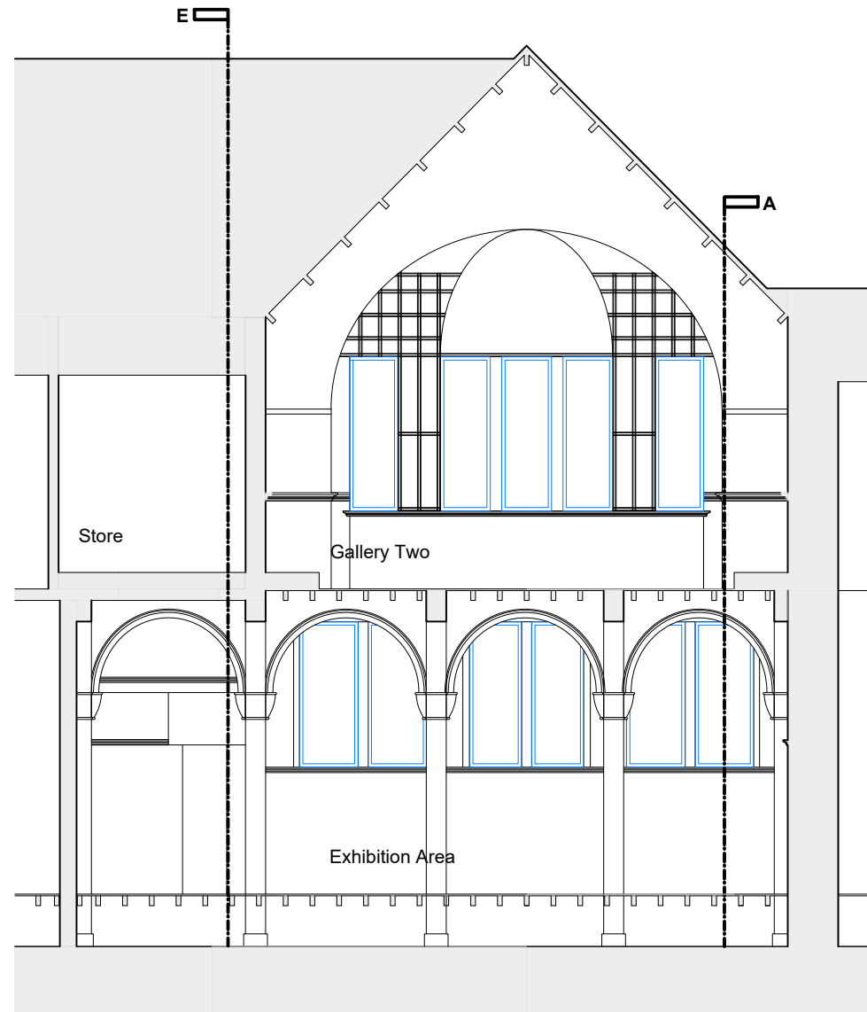
01 Section D-D - As Existing L(01)05 1:100
