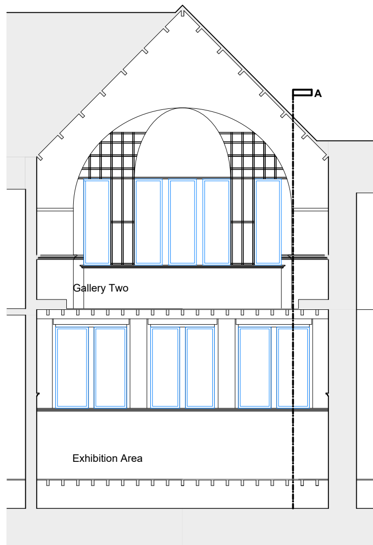
01 Section B-B - As Existing L(01)04 1:100
