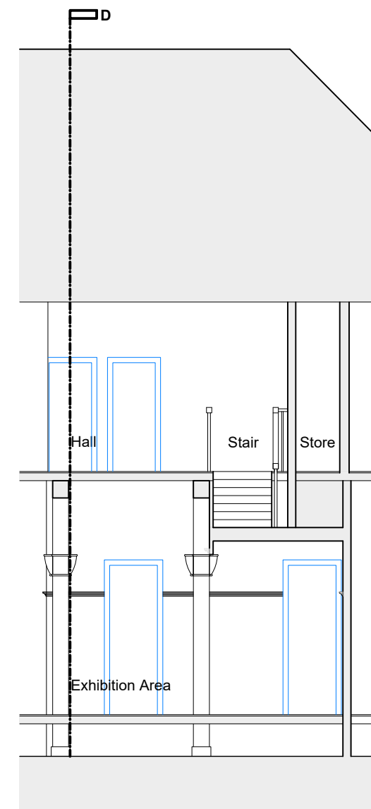
01 Section C-C - As Existing L(01)04 1:100
