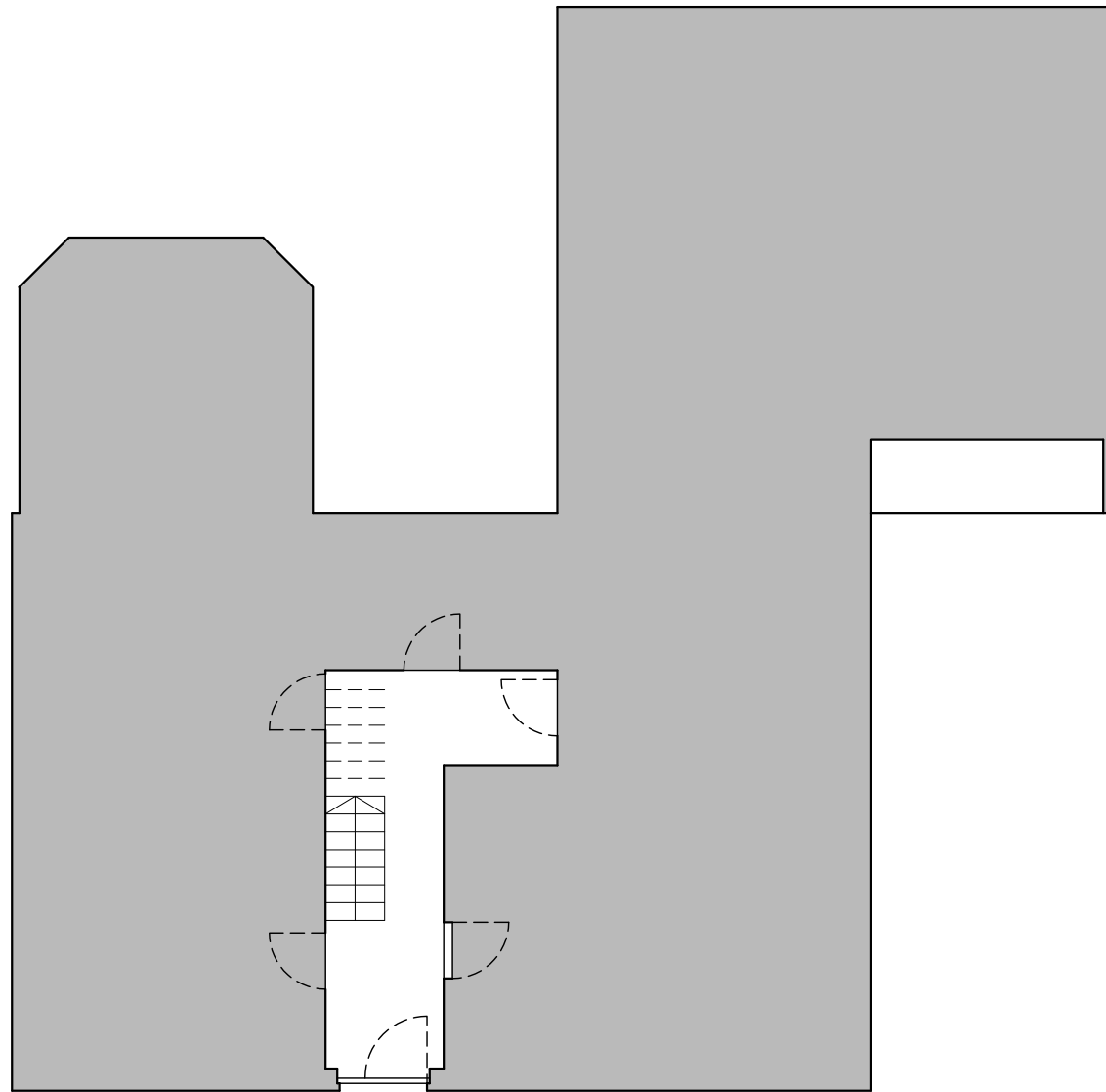
01 Ground Floor Plan - As existing (01)01 1:100
