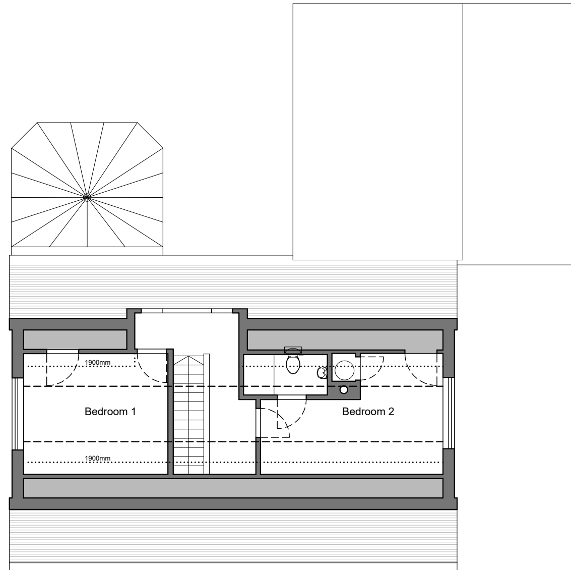
02 First Floor Plan - As existing (01)01 1:100
