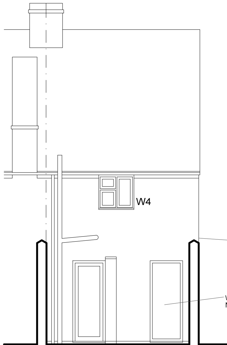
REAR ELEVATION (Elevation 'C' on Block Plan) PROPOSED
