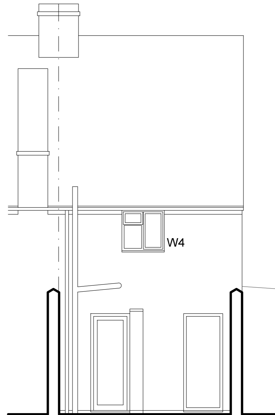
REAR ELEVATION (Elevation 'C' on Block Plan) EXISTING
