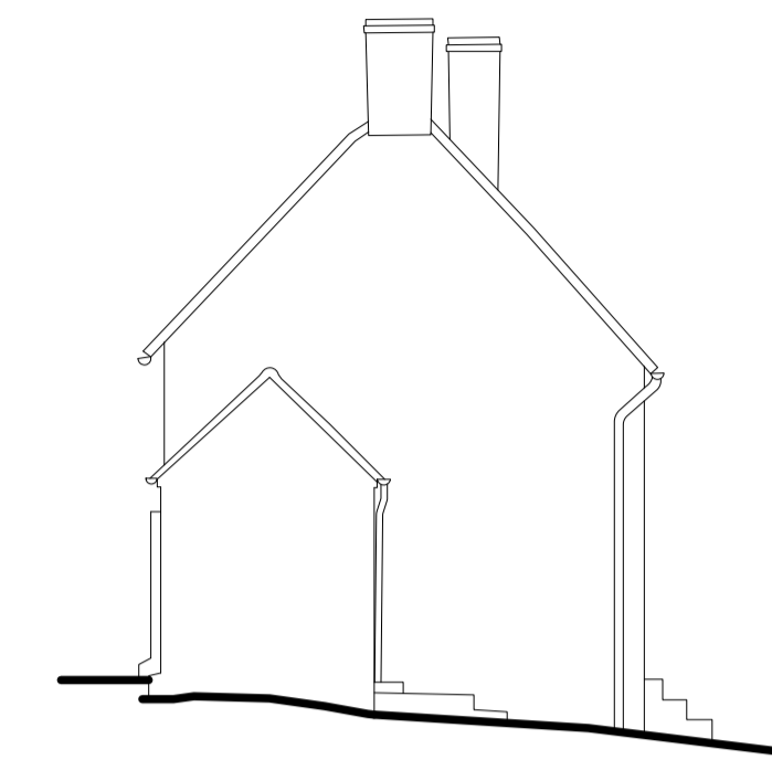
West elevation
