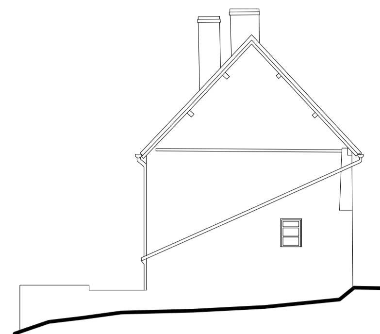
East elevation
