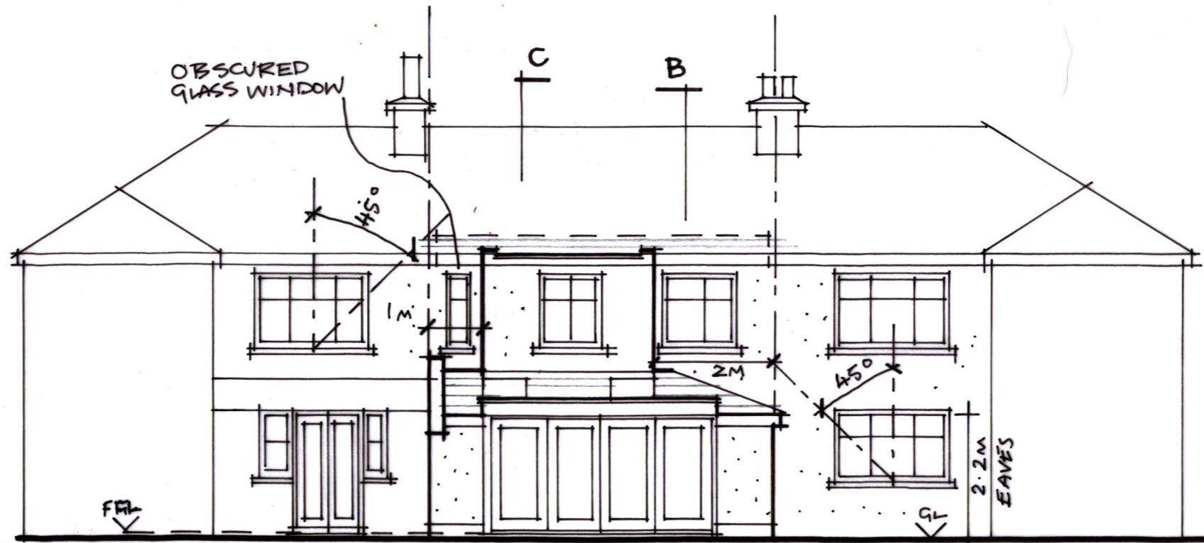
REVISED REAR ELEVATION
