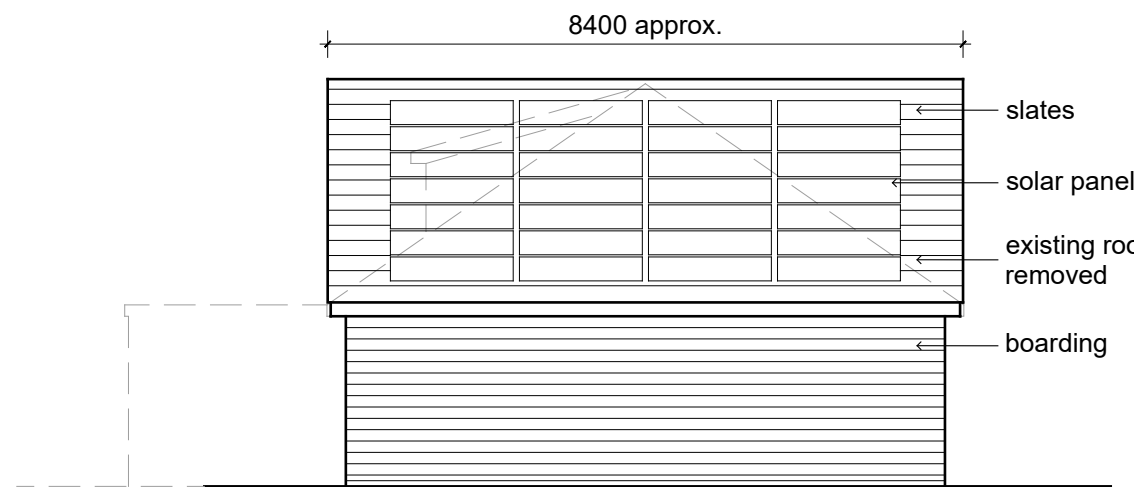
side elevation
