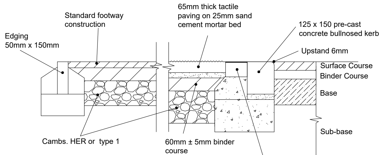
Typical Section
