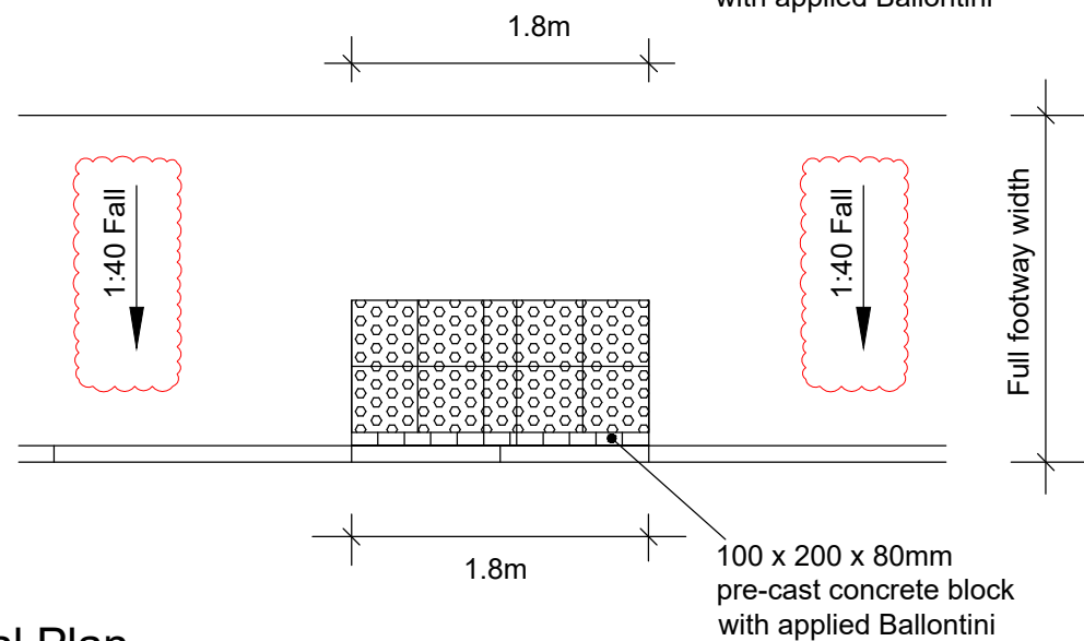
Typical Plan
