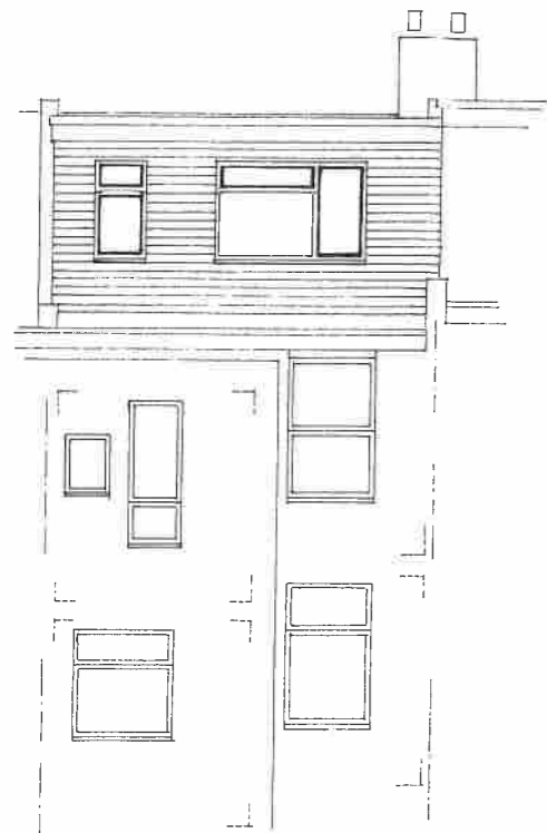
REAR [ EAST ] ELEVATION
