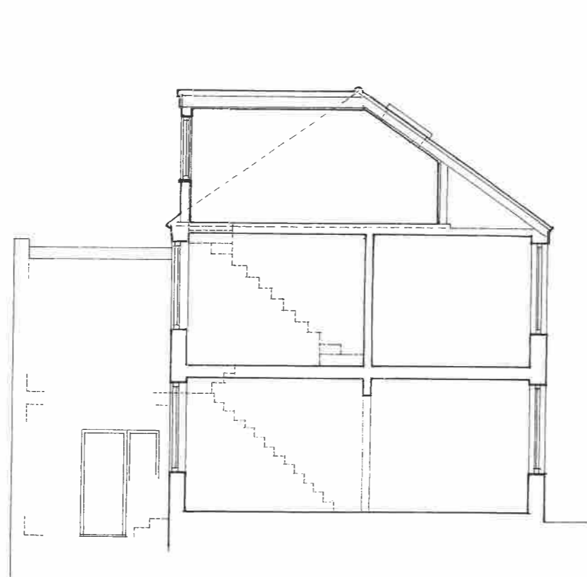
SECTION B-B
