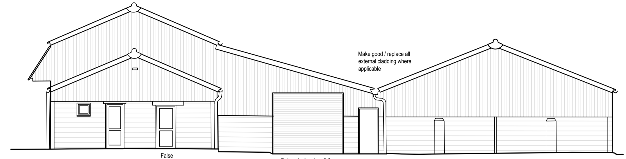
East Elevation
