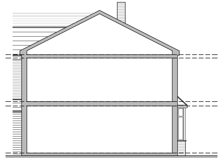
LEFT ELEVATION 1:100
