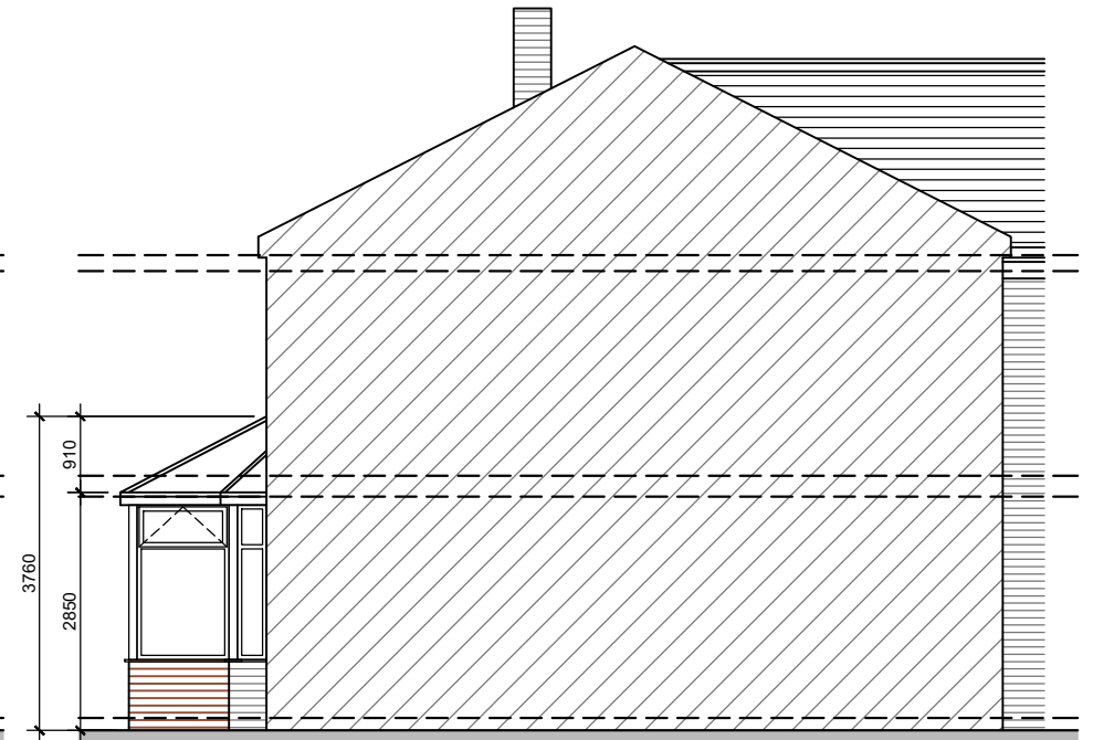
RIGHT ELEVATION 1:100
