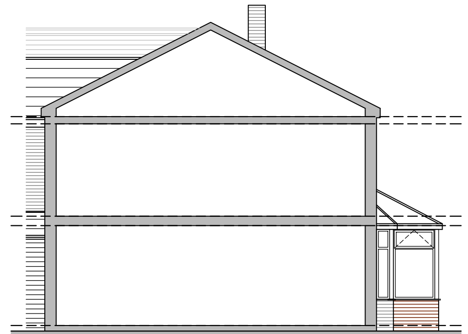
LEFT ELEVATION 1:100
